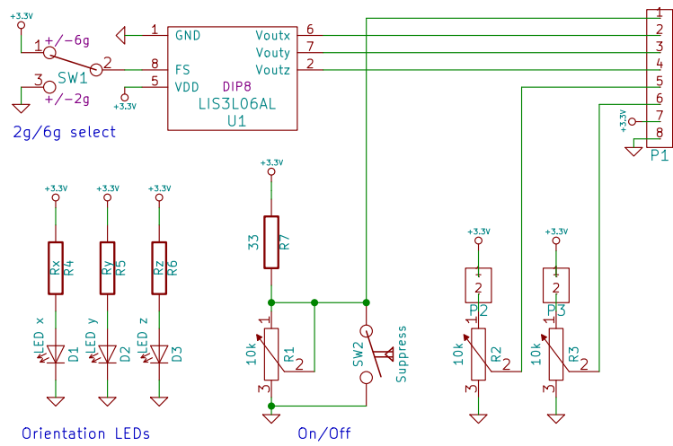
Auxiliary Pots / Ext. Sensor Connectors
